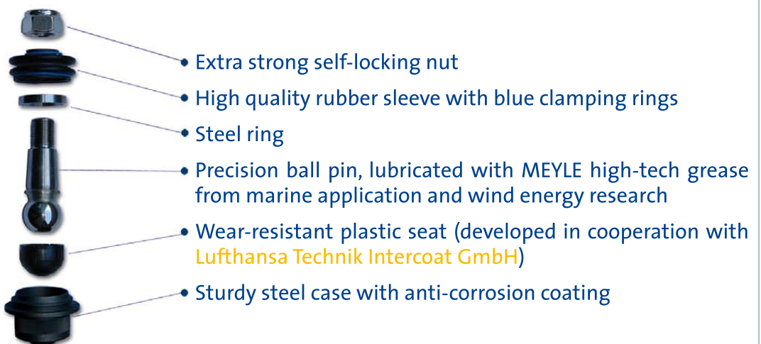
Exploded drawing ball joint
